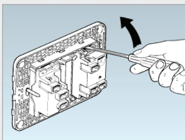
Removal with use of a tool, possible also from the front of the device.
